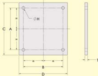
Location plate for Types BA, BB, BT & BW
