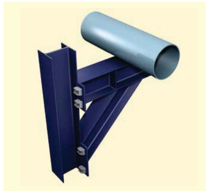
Typical end plate cantilevered connection supporting heavy duty pipe work.
