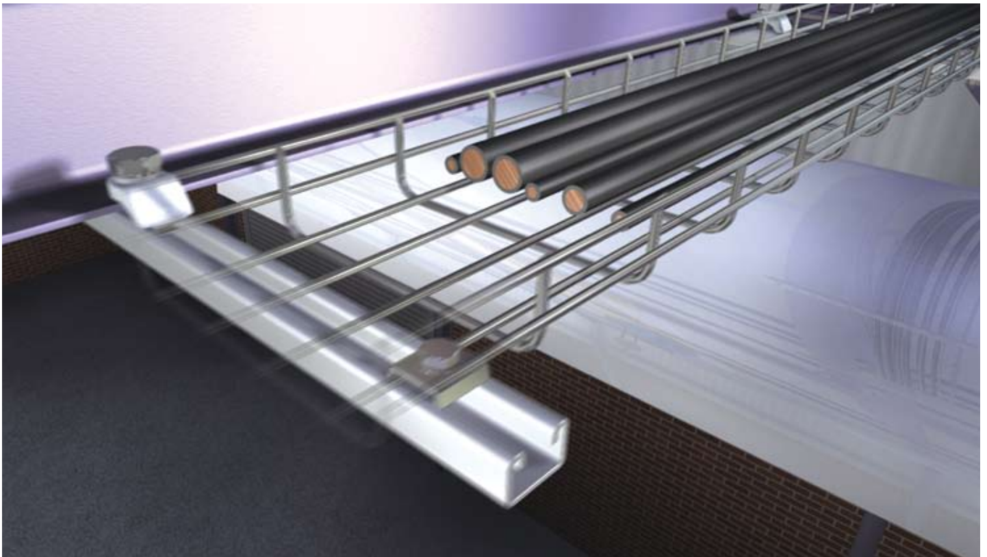
Cable tray support to existing steel
